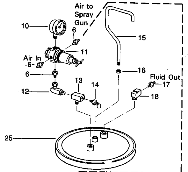
PT-511-WB & PT-521-WB PRESSURE TANK (Dual Regulation included with these models)
