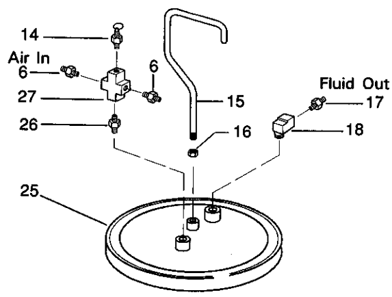
PT-500-WB PRESSURE TANK (Includes Ref. No. 1, 2 and 19 thru 24)
