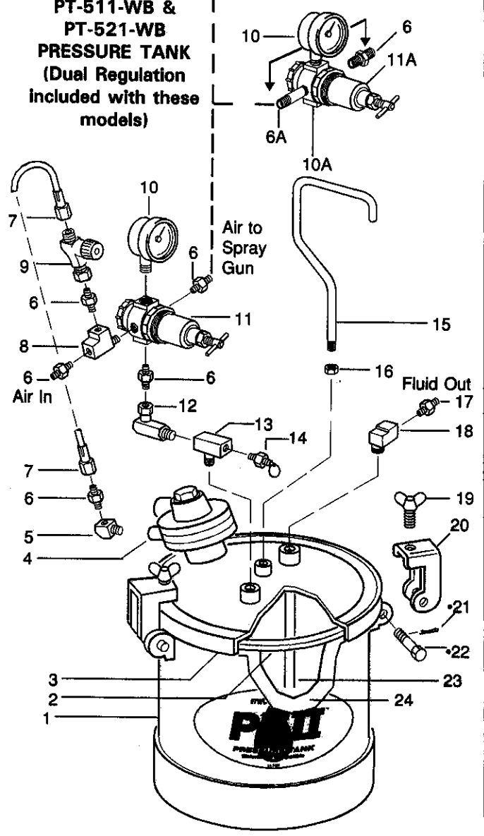
PT-520-WB PRESSURE TANK WITH AGITATOR
